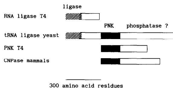
Fig. 3. A tentative scheme of the domainal organization of the CNPases and the tRNA processing enzymes. Regions of sequence similarity are highlighted by identical hatching.
